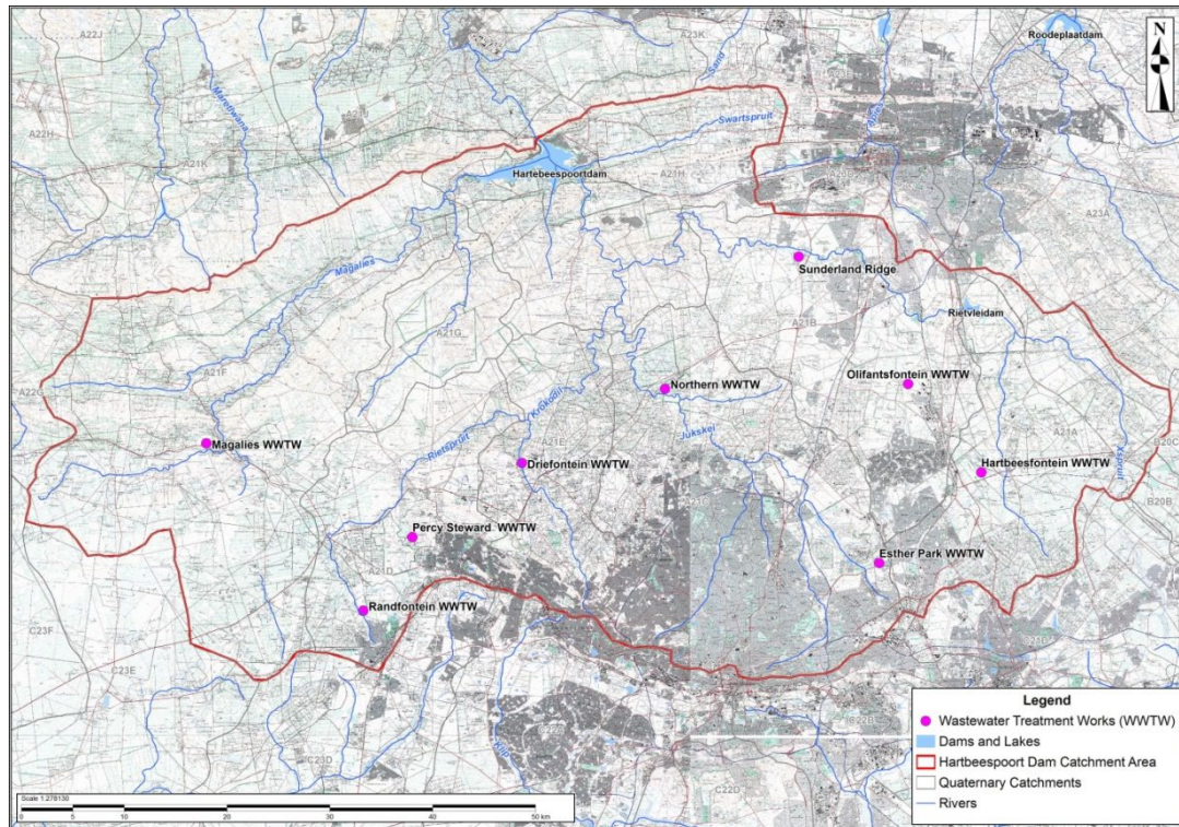
Figure 3: Location of WWTWs in the Hartbeespoort Catchment
